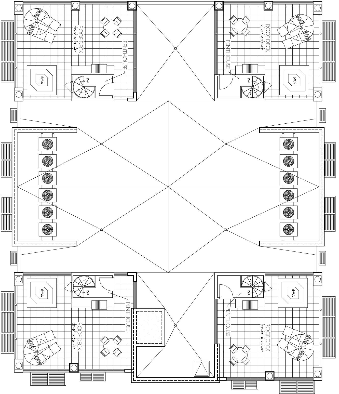
SUN DECK / ROOF PLAN
